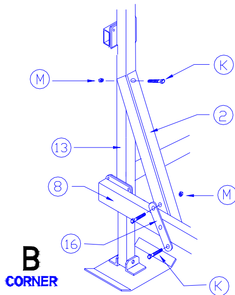
Figure 3-7 Lower Diagonal Brace Assembly
