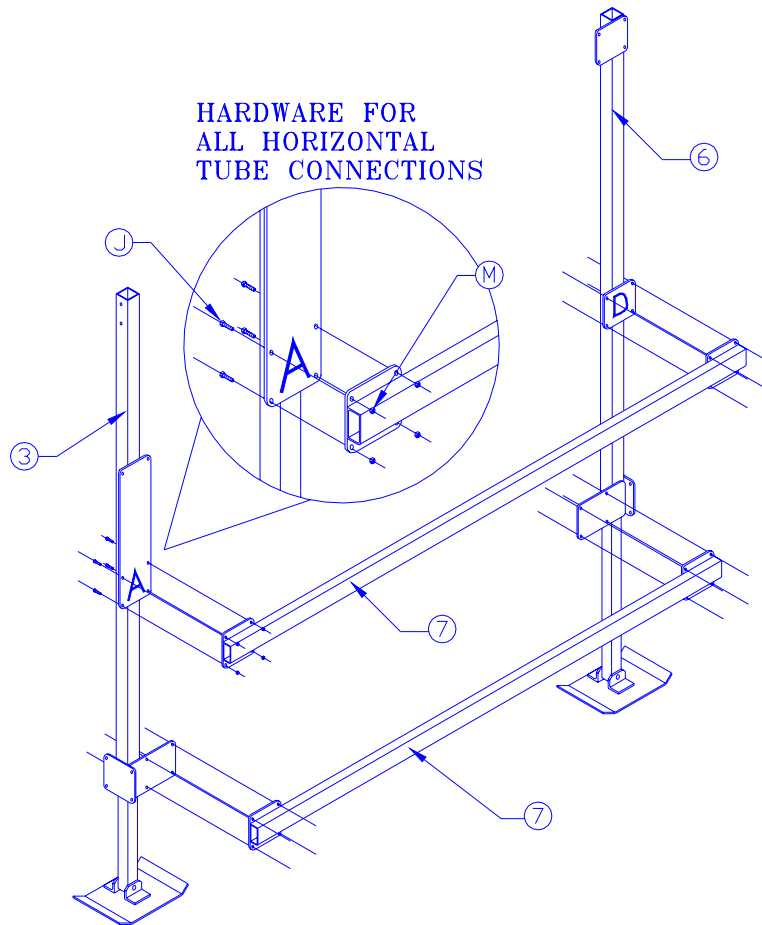
Figure 3-4 Frame Side Assembly
