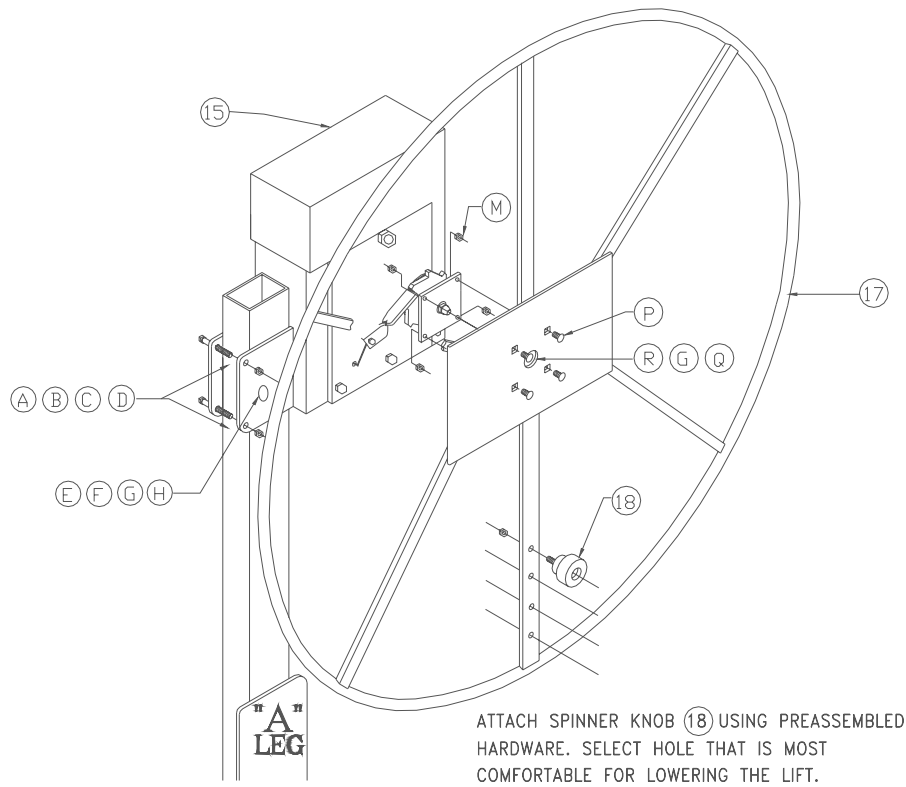
Figure 3-9 VL Handwheel Mounting
