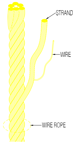
Figure 5-1. Wire Rope Components
