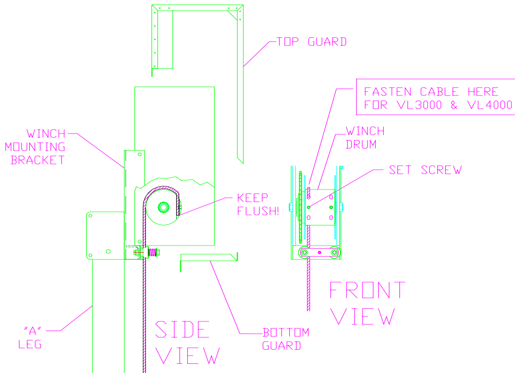
Figure 3-10 Winch Cable Reeving
