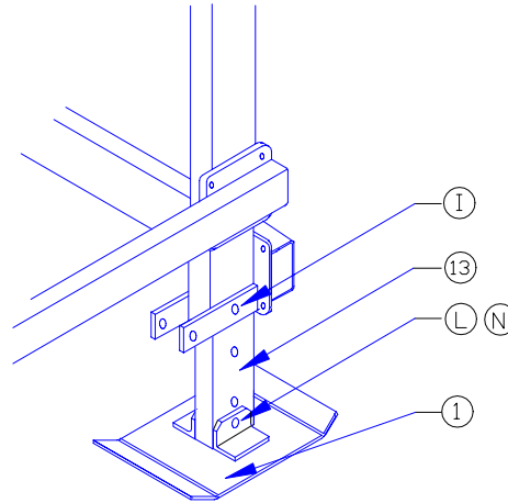
Figure 3-3 Vertical Leg Assembly
